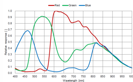
MV-CU004-10GC
