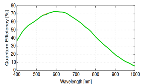
MV-CS032-10GM
